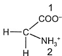
glycine
