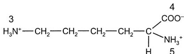
lysine
