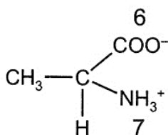
alanine
